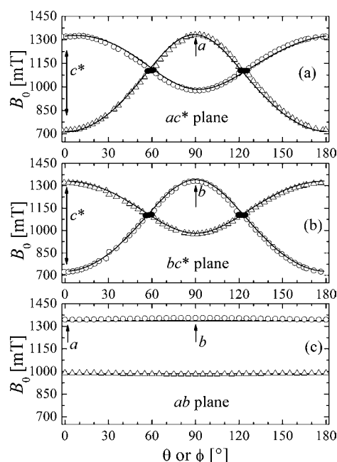
Figure 6. Angular dependence of the allowed S_z = 0 \leftrightarrow \pm 1 transitions observed with B_0 in the (a) ac *, (b) bc *, and (c) ab planes. Symbols and the solid lines are experimental and fitting data, respectively.
